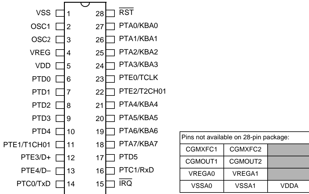
Figure 1-3. 28-Pin SOIC Pin Assignment
