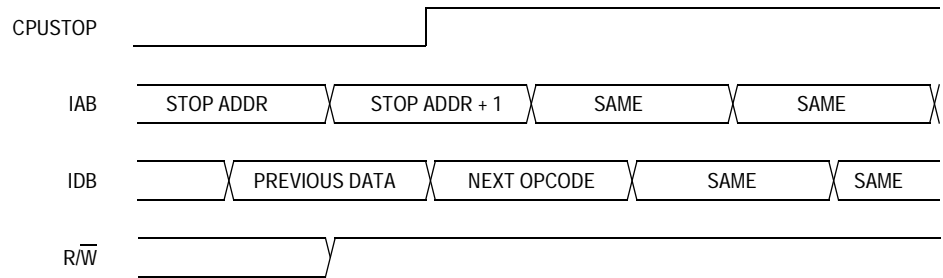
Figure 8-17. Stop Mode Entry Timing
