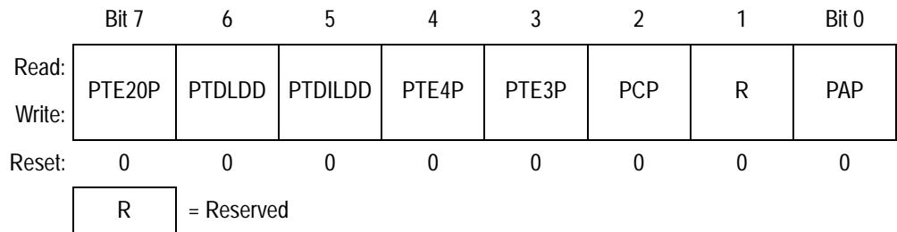
Figure 14-14. Port Option Control Register (POCR)
