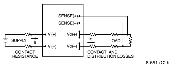
Figure 15. Effective Circuit Configuration for Single-Module Remote-Sense Operation
