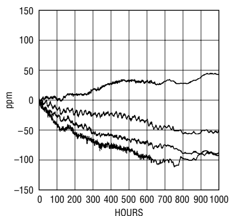
Figure 5. Typical Long-Term Drift
