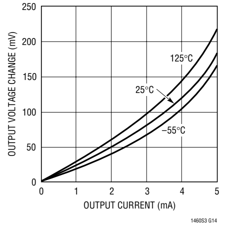
10V Load Regulation, Sinking
