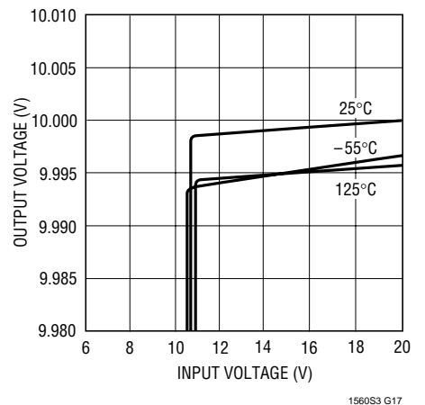
10V Line Regulation
