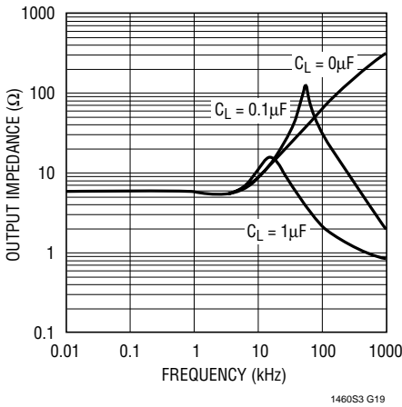
10V Output Impedance vs Frequency
