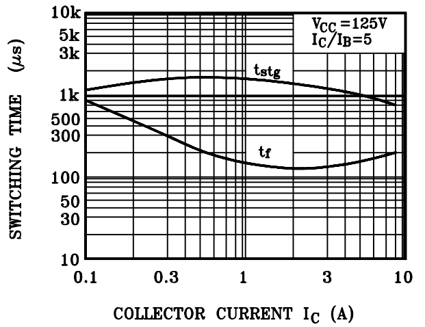
SWITCHING CHARACTERISTIC
