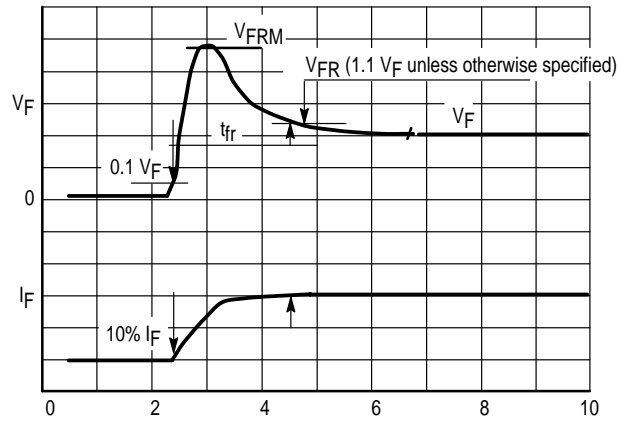
Figure 27. t_{fr} Measurements
