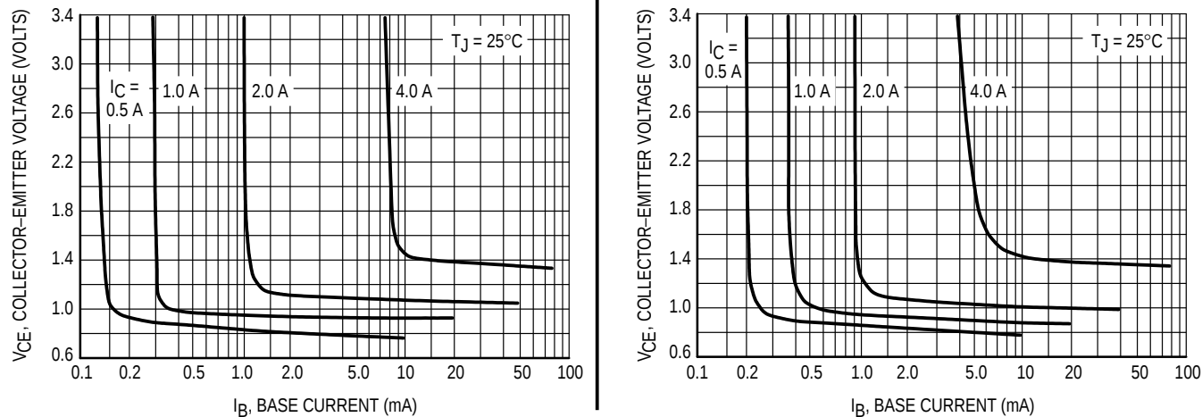
Figure 11. Collector Saturation Region
