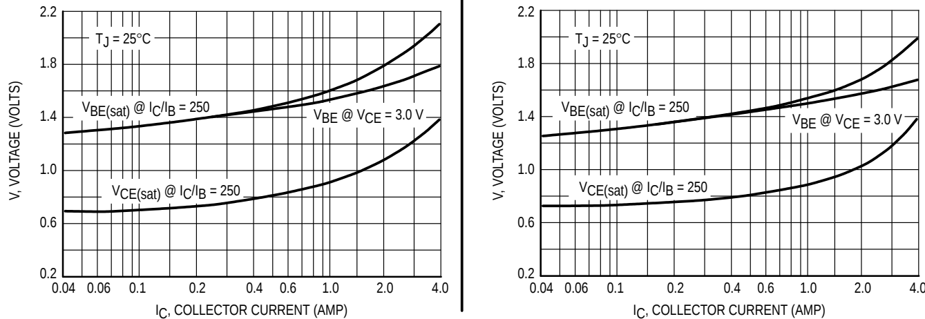
Figure 12. "On" Voltages
