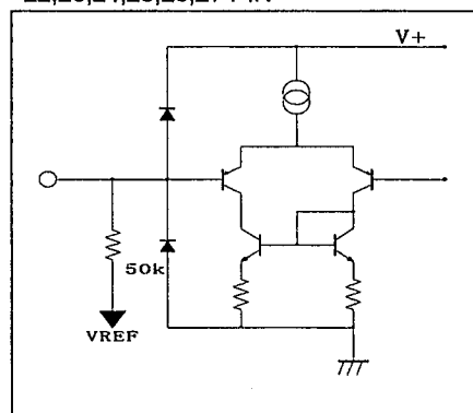
22,23,24,25,26,27 PIN
