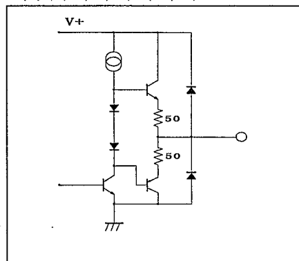
4,7,8,9,10,11,12,15,17,21,28 PIN
