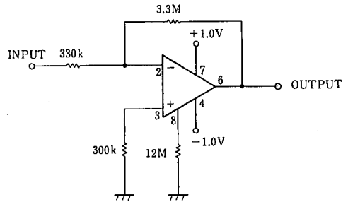
500nW, 10times Inverting Amplifier
