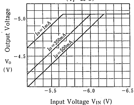
NJM79M05 Dropout Characteristics
