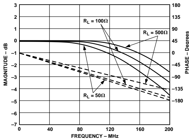
Figure 8. Frequency Response vs. R_{LOAD}
