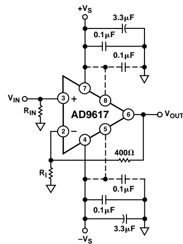
Figure 20. Noninverting Operation
