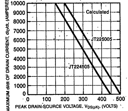
MAXIMUM TURN-OFF di/dt VS. PEAK DRAIN-SOURCE VOLTAGE
