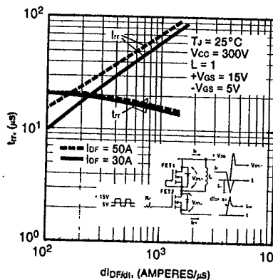
SOURCE-DRAIN DIODE REVERSE RECOVERY CHARACTERISTICS (TYPICAL FOR HALF BRIDGE OPERATION)
