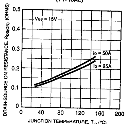
ON-RESISTANCE VS. TEMPERATURE (TYPICAL)
