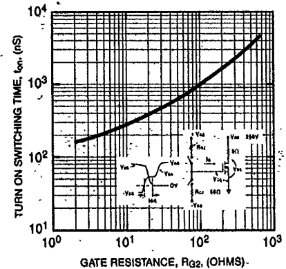
TURN-ON SPEED VS. GATE RESISTANCE (TYPICAL)
