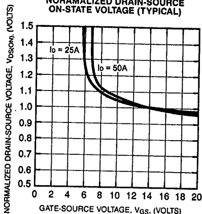
NORAMALIZED DRAIN-SOURCE ON-STATE VOLTAGE (TYPICAL)
