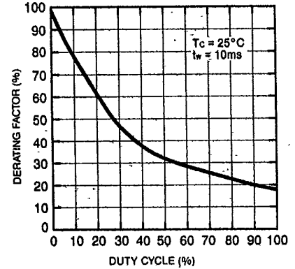
DUTY CYCLE DERATING FACTOR OF SAFE OPERATING AREA (S.O.A.)
