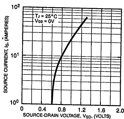
SOURCE-DRAIN DIODE FORWARD CHARACTERISTICS (TYPICAL)
