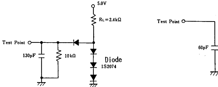
DB 0 to DB 7 load circuit
