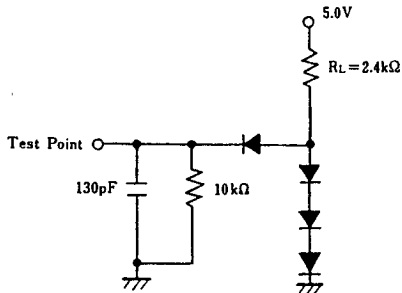
DB 0 to DB 7 load circuit
