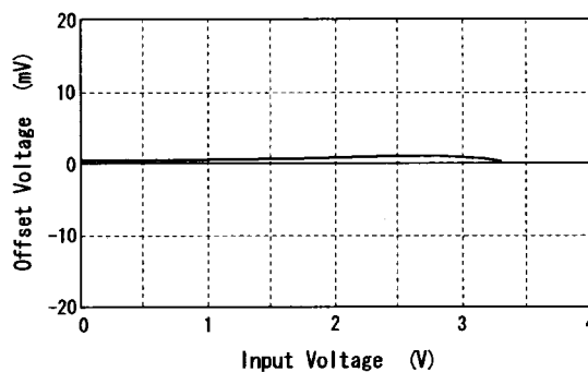
Offset Voltage vs. Input Voltage
