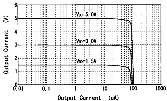
Output Voltage vs. Output Current (SOURCE)
