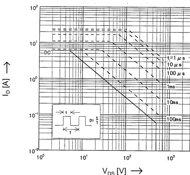
Safe operation area I_D = f(V_{DS}) ; D = 0.01 ; T_{ch} = 25^\circ\text{C}
