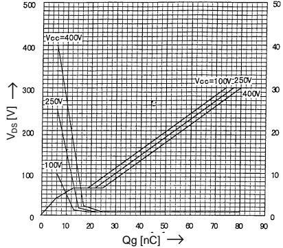
Typical Gate Charge Characteristic V_{GS} = f(Q_g) ; I_D = 6\text{A} ; T_{ch} = 25^\circ\text{C}
