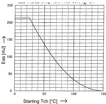
Avalanche Energy Derating E_{as} = f(\text{starting } T_{ch}) ; V_{CC} = 50\text{V} ; I_{AV} = 6\text{A}
