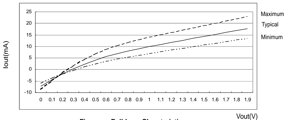
Figure a : Pulldown Charateristics
