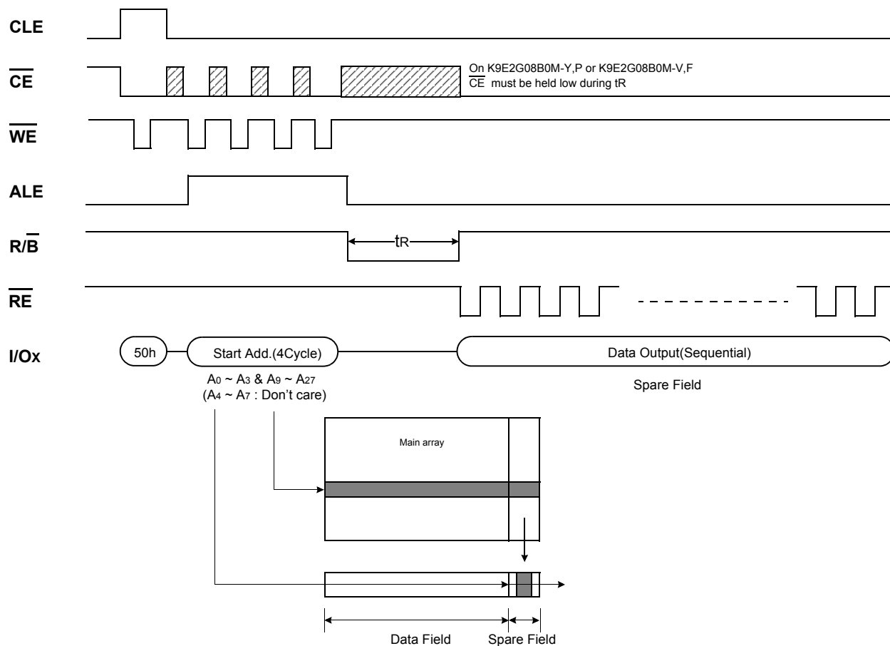
Figure 8-2. Read2 Operation
