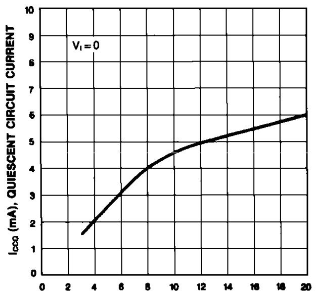
QUIESCENT CIRCUIT CURRENT-SUPPLY VOLTAGE
