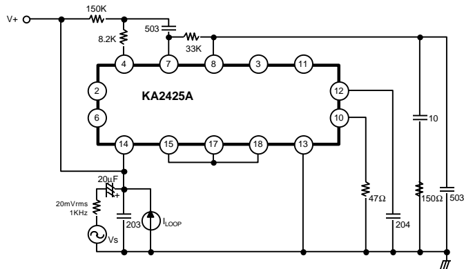
Fig 4. AC Impedance, Receive and Sidetone Rejection Test
