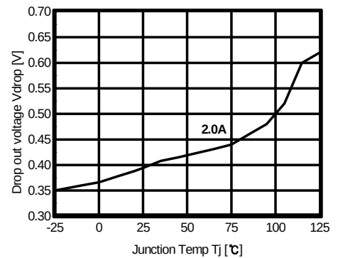
Figure 5. Dropout Voltage vs. Junction Temperature
