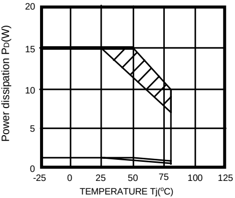
Figure 6. Power Dissipation vs. Temperature(Tj)
