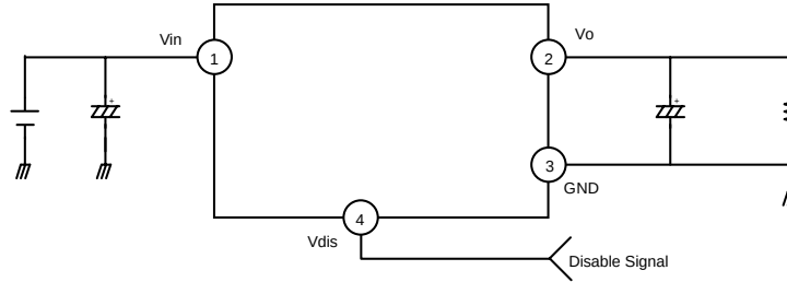
Figure 1. Application Circuit
