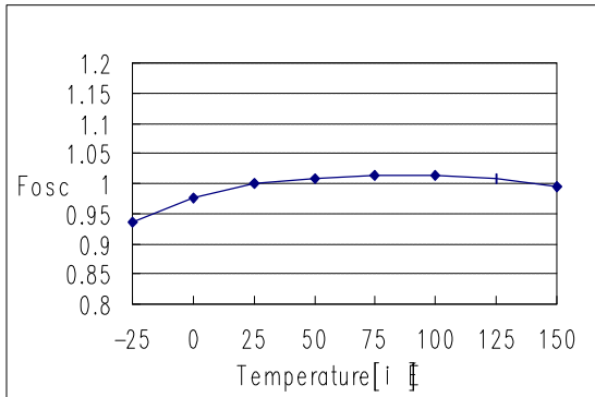
Figure 1. Operating Frequency
