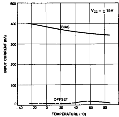
Figure 1. Input Current
