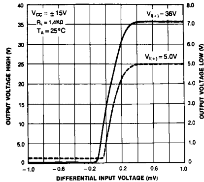
Figure 3. Transfer Function
