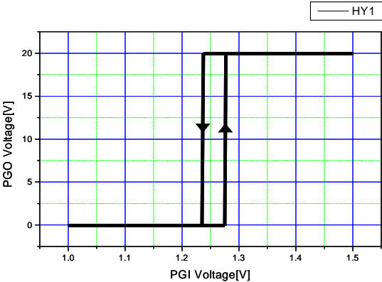
Figure 7. Hysteresis Voltage 1
