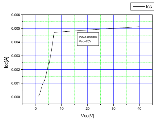
Figure 1. Vcc - Icc
