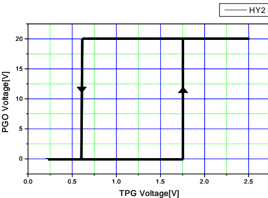
Figure 8. Hysteresis Voltage 2
