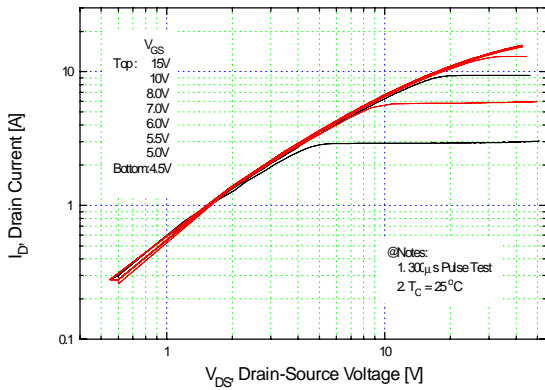
Fig 1. Output Characteristics
