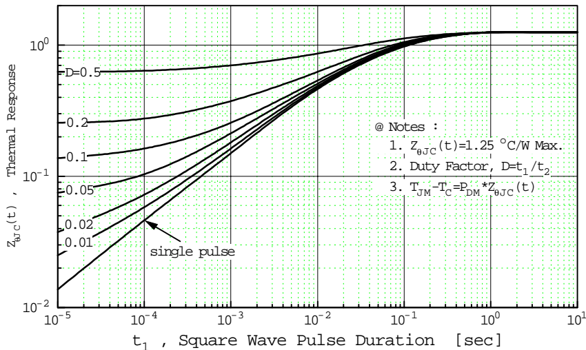
Fig. 11 Thermal Response
