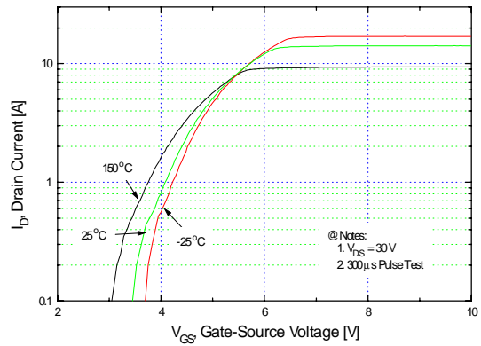
Fig. 2 Transfer Characteristics
