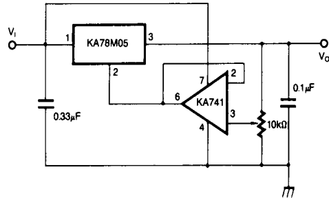
Figure 4. Adjustable Output Regulator (7 to 30V)
