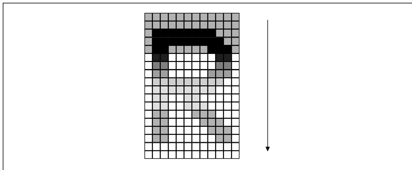
Figure 20. Scrolling
