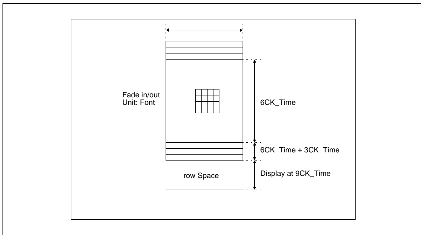
Figure 21. Fade-In/Fade-Out
