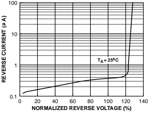
Reverse Characteristics
