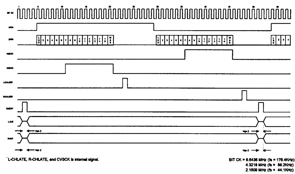
TIMING DIAGRAM 2 (When MS = "L")
