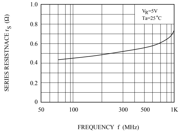
r_s - f
