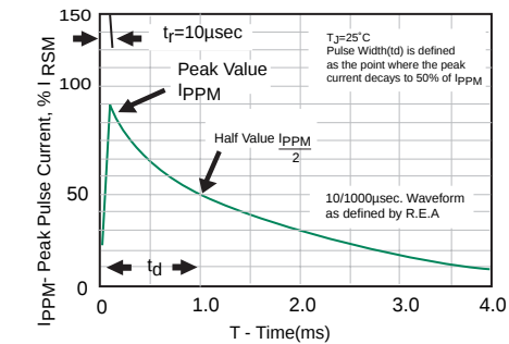
Fig. 3 Pulse Waveform
