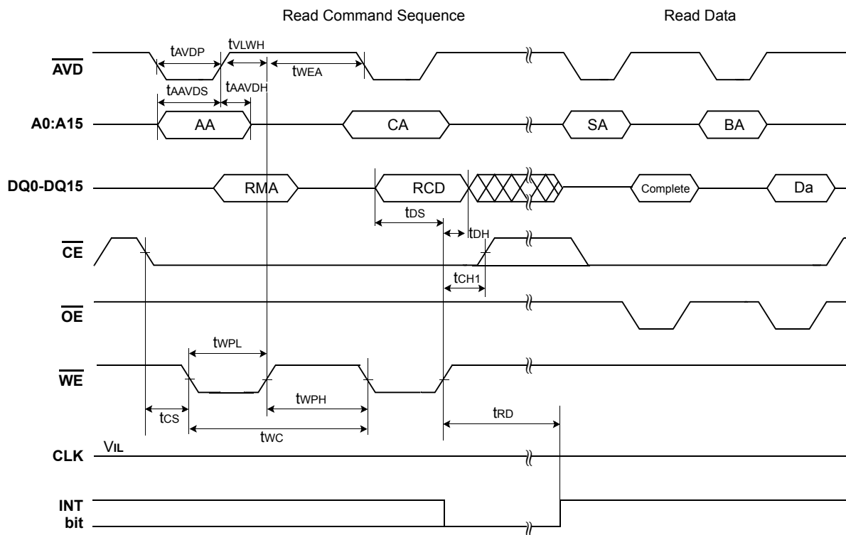
Figure 36. Load Operation Timing
