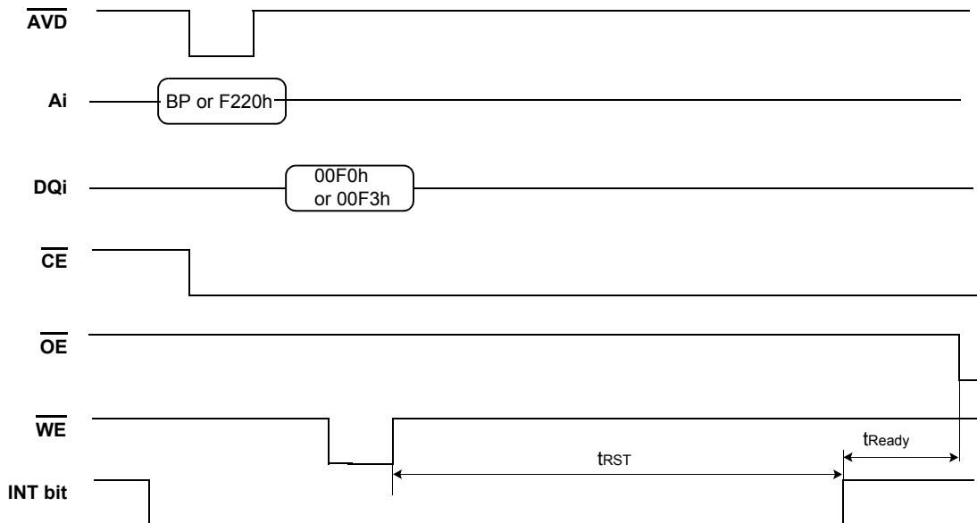
Figure 35. Reset Timing
