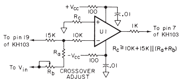
Figure 4: Inverting Gain Composite Amplifier to be Used with Figure 2 Circuit
