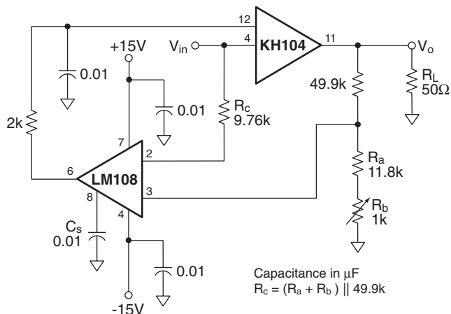
Figure 2: Composite Amplifier
