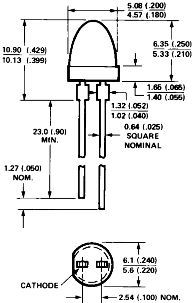
PACKAGE OUTLINE "B" HLMP-3390, -3490, -3590
