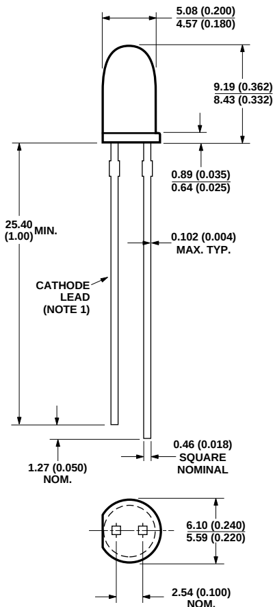
PACKAGE OUTLINE "D" HLMP-DC40
