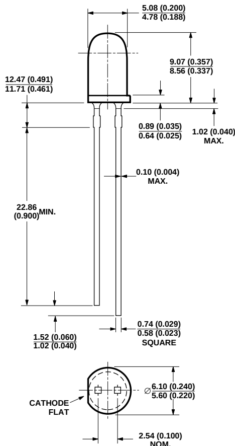
PACKAGE OUTLINE "E" HLMP-DC40
