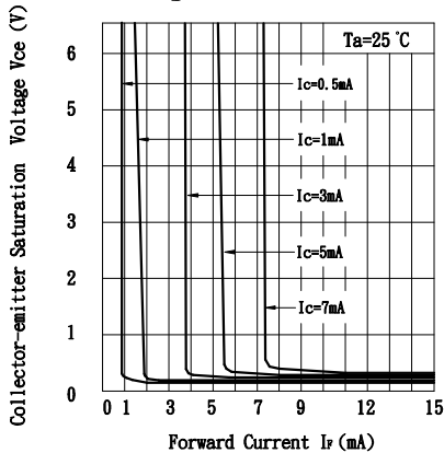
Fig. 9 Collector-emitter Saturation Voltage vs. Forward Current
