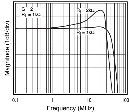
Figure 2: Frequency Response vs. R_f
