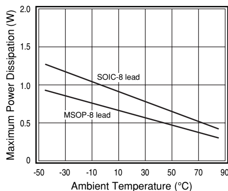
Figure 2: Power Derating Curves
