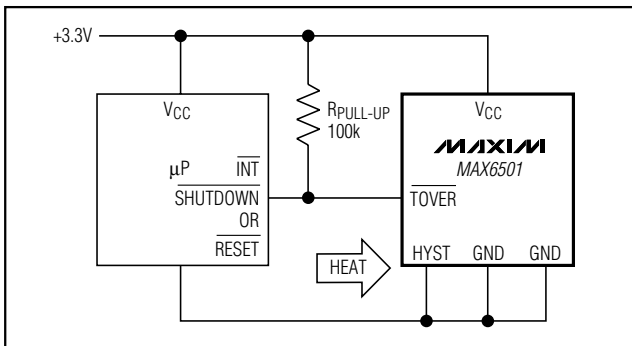
Figure 2. Microprocessor Alarm/Reset
