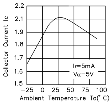
Fig.3 Collector Current vs. Ambient Temperature
