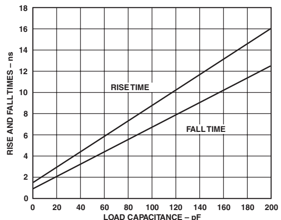
Figure 7. Typical Rise and Fall Time (10% 90% V)
