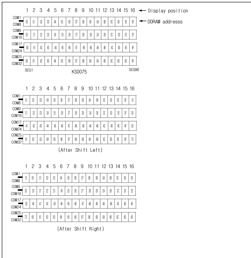
Fig-7. 4-line X 16ch. display (6-dot font width)
