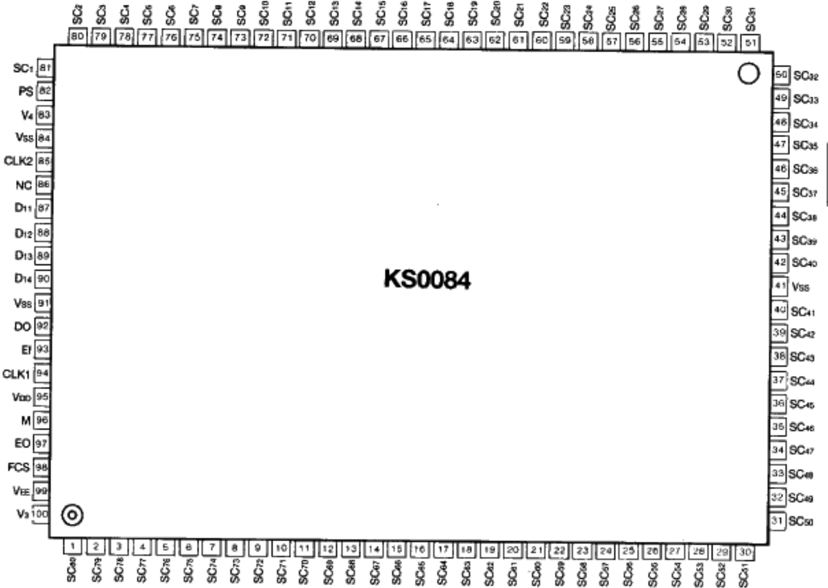
Fig.3 100QFP Top View.
