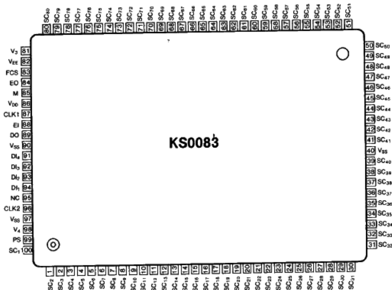
Fig. 2. 100 QFP Top View
