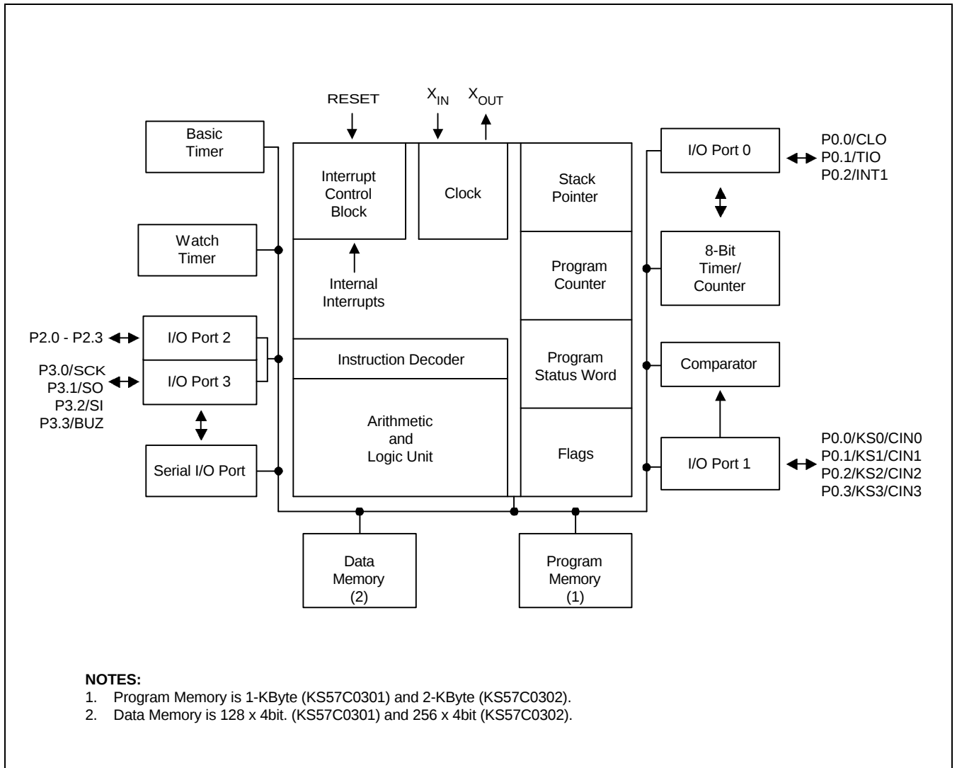
Figure 1-1. KS57C0301/0302 Block Diagram
