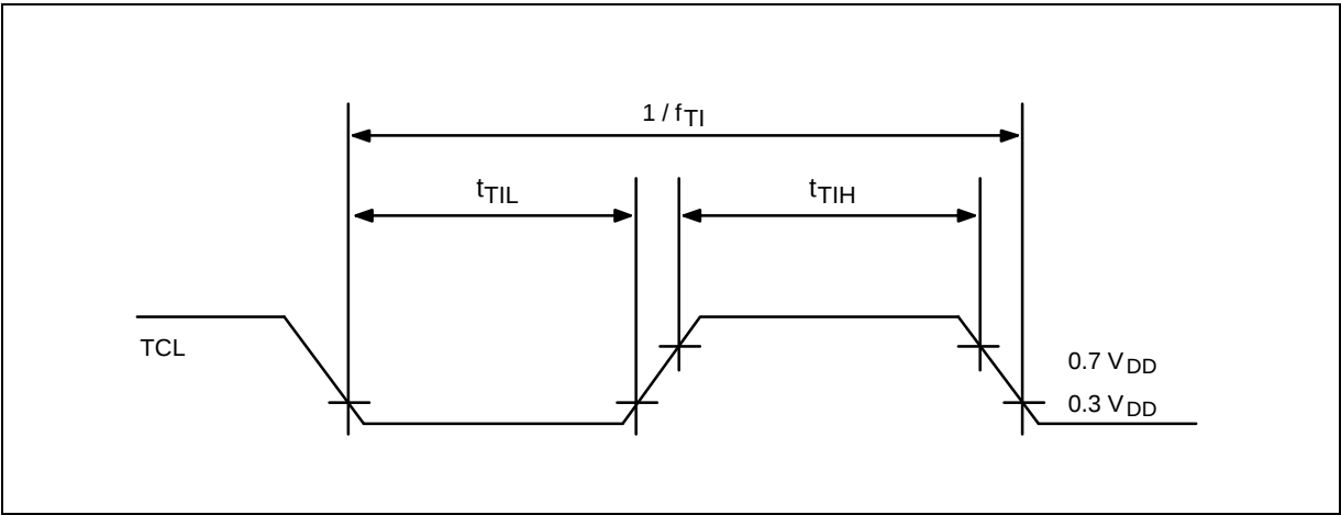
Figure 14-6. TCL Timing
