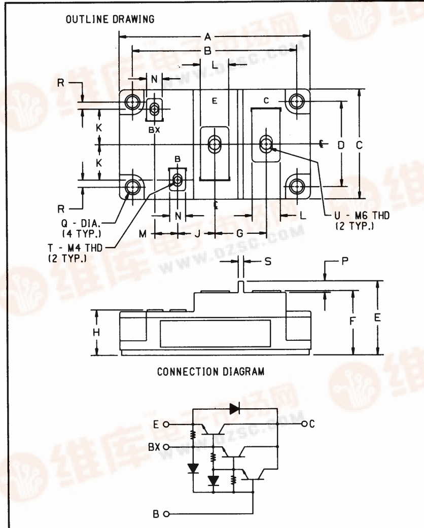
Outline Drawing
