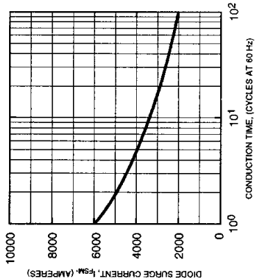
DIODE FORWARD SURGE CURRENT
