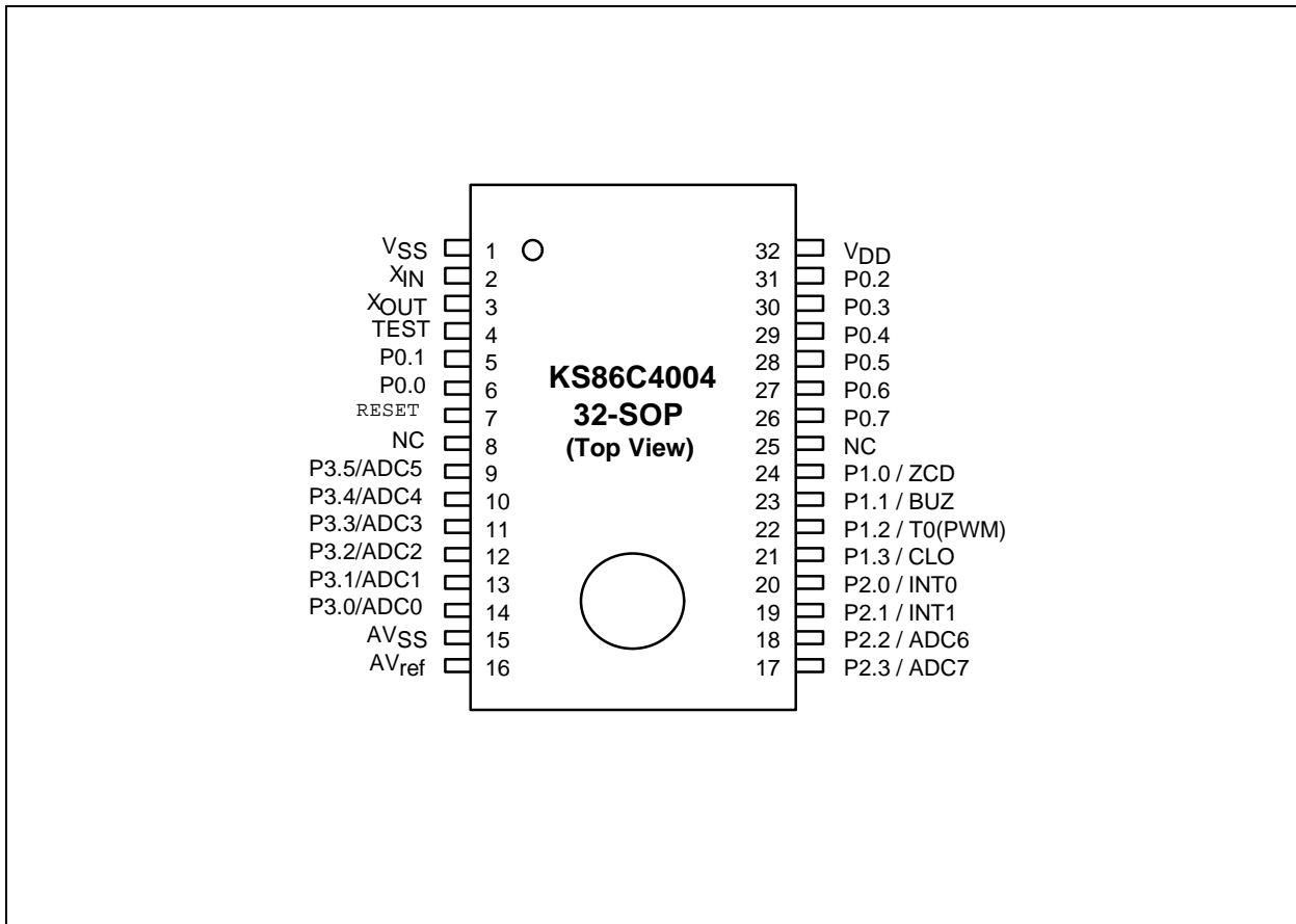
Figure 1-3. Pin Assignment Diagram (32-Pin SOP Package)
