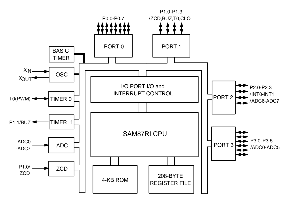
Figure 1-1. Block Diagram
