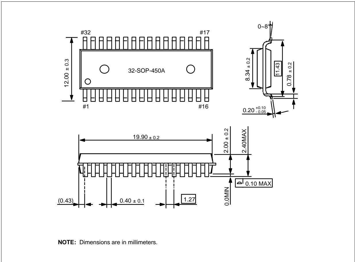
Figure 14-2. 32-SOP-450A Package Dimensions
