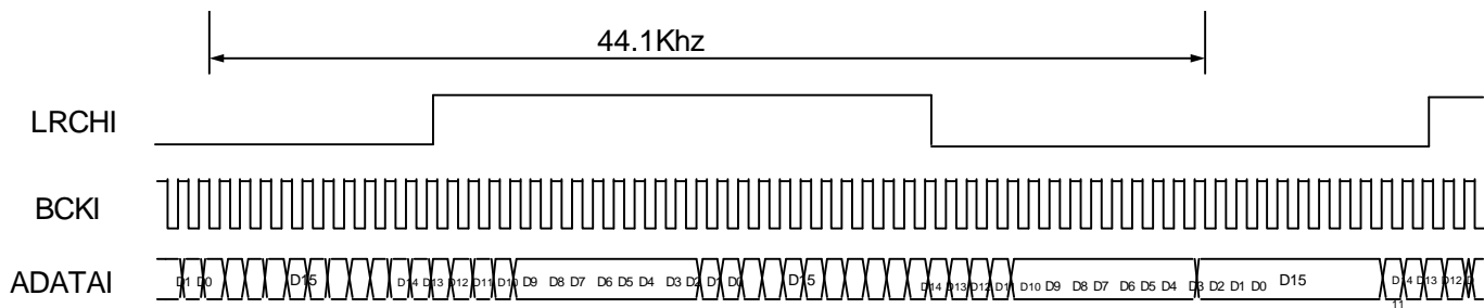
Fig.21. Timing chart of signal ESP IC outputting to DSP
