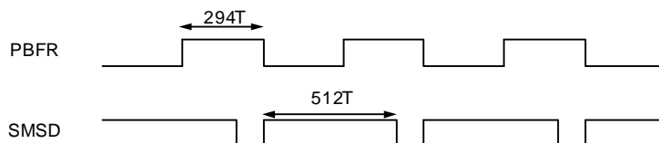
(B) Timing chart of SMDS when PBFR is 294T
