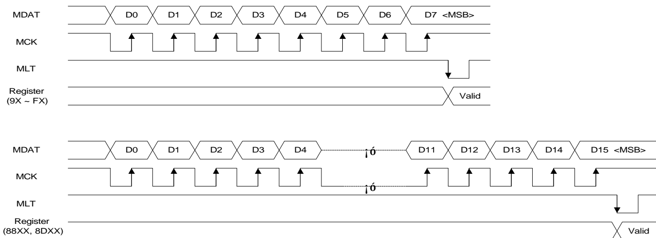
Fig.1. Micom data input timing chart
