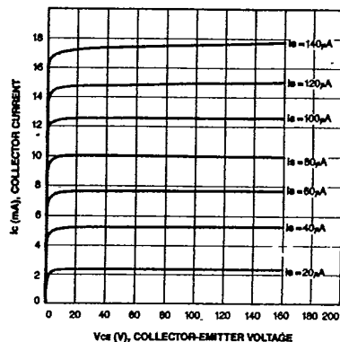
STATIC CHARACTERISTIC
